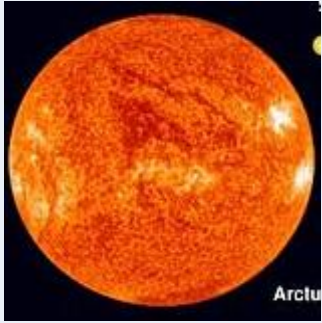
Arcturus
