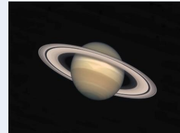
Saturne
